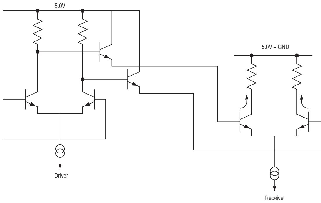
Figure 6. Generic Driver/Receiver Pair
