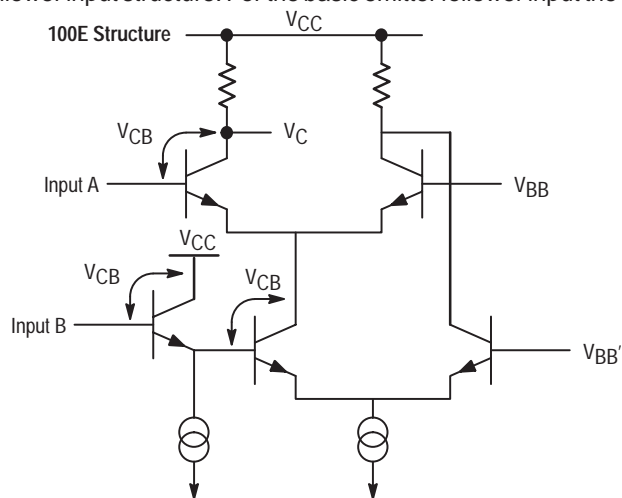
Figure 3. Emitter Follower Series Gate Input Structure
