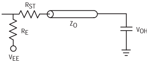
Figure 3.21. Equivalent Circuit with Output Cutoff
