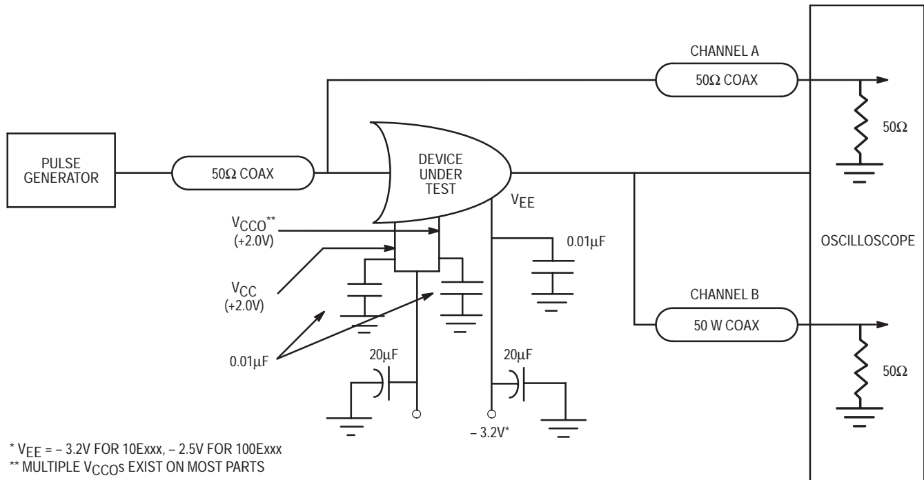
Figure 2.8. Typical ECLinPS Test Setup
