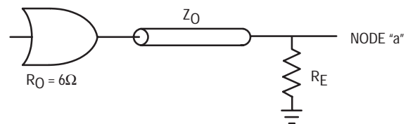
Figure 2.1. Typical Transmission Line Driving Scenario
