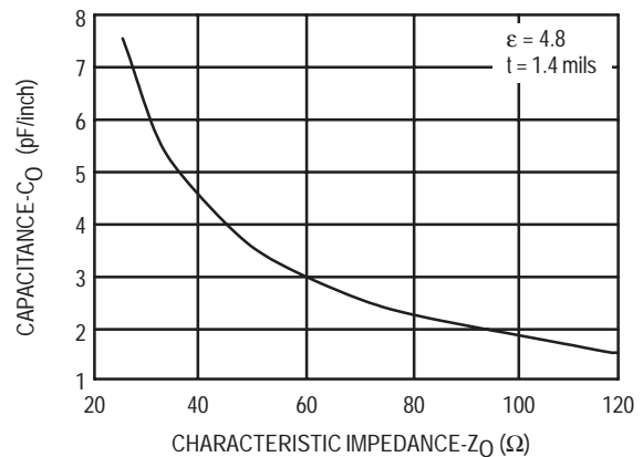
Figure 3.7. Stripline Capacitance vs Impedance and Trace Width
