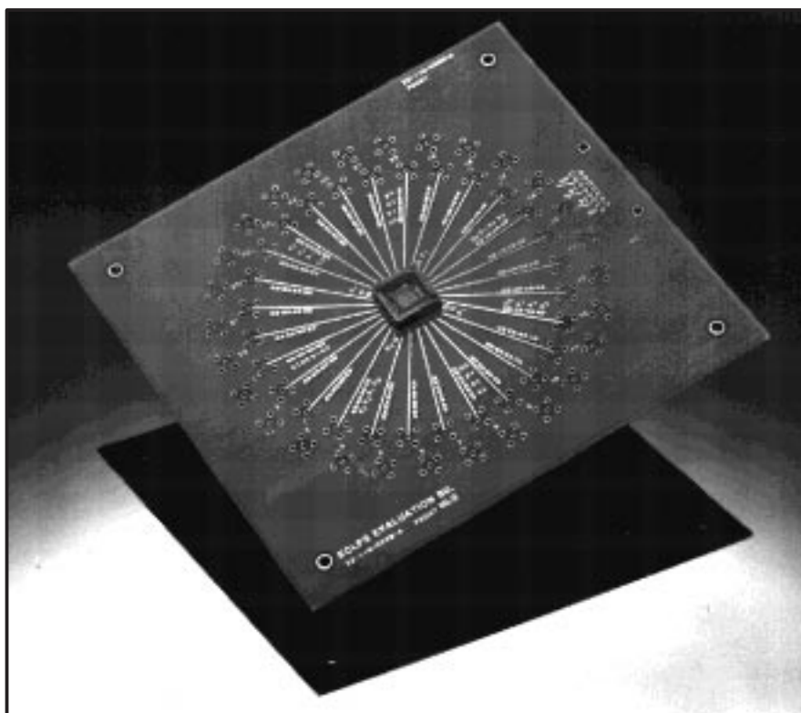
Figure 2.9. ECLinPS AC Test Board
