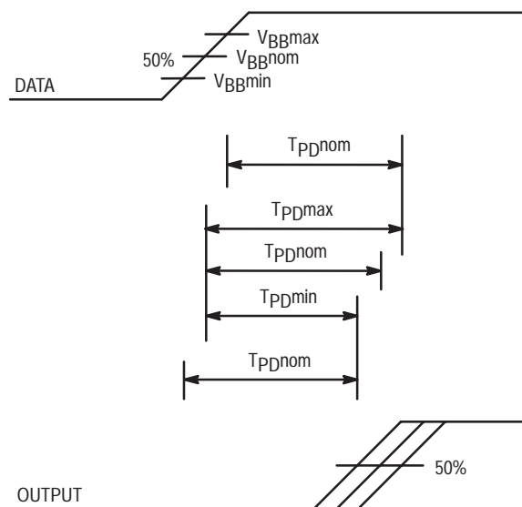
Figure 1.3. Delay vs Switching Reference Offset
