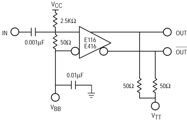
Figure 4.4. AC Couple Circuit with DC Offset
