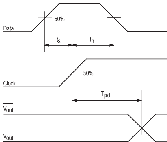
Figure 2.5. Set-Up and Hold Waveforms
