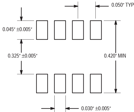
Figure 4. 20-Lead Wide SOIC Solder Pad Dimensions
