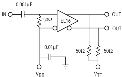
Figure 2. AC Coupling Architecture
