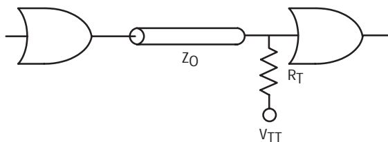
FIGURE 3.13A PARALLEL TERMINATION TO V TT
