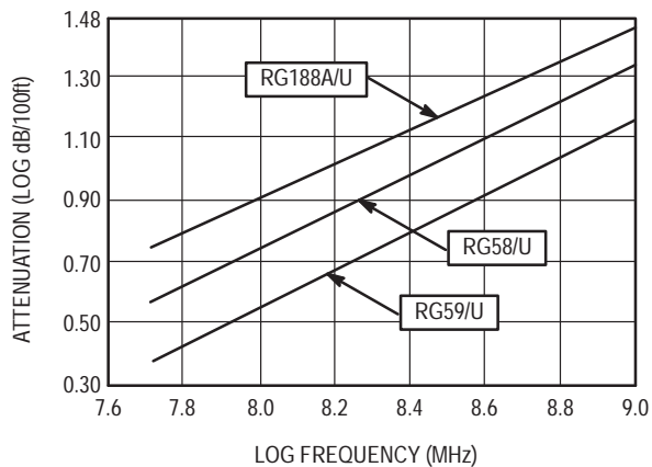
Figure 3.11. Coaxial Cable Attenuation vs Frequency
