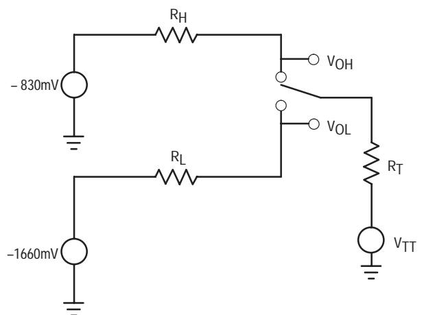
Figure 3.16. Equivalent Circuit for Calculating 100E Output Levels
