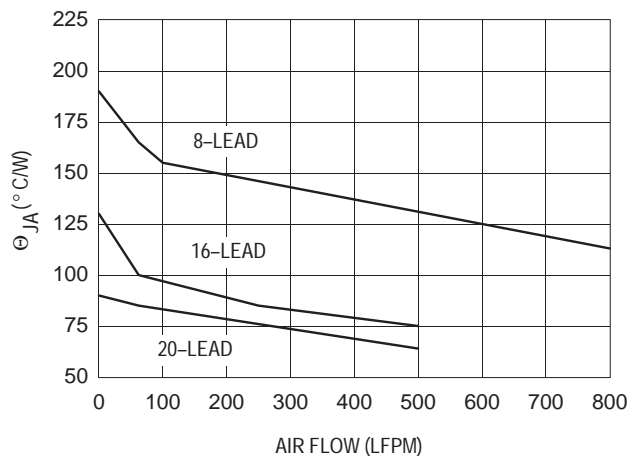
Figure 5. SOIC Thermal Resistance
