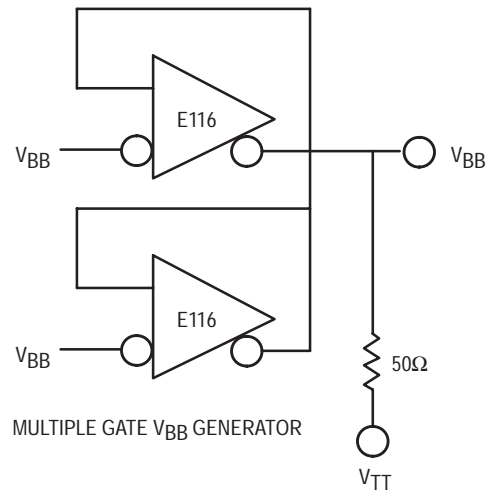
Figure 4.5. High Current V_{BB} Generator
