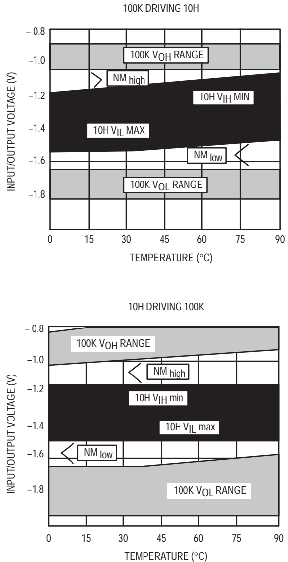
Figure 4.1. Interfacing 10H ECL and 100K ECL Clock inputs on flip-flop devices in the ECLinPS family are especially sensitive to slow edge rates. Flip-flops have been successfully clocked in a noise free bench setup environment with edge rates of up to 20ns. However, in ATE systems where more noise is present, clocking problems arise with input edge rates of greater than 6.0 or 7.0ns. To ensure reliable operation in a system with input clock edges slower than 7.0ns, it is recommended that the signals be buffered
