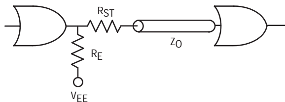
Figure 3.18. Series Termination
