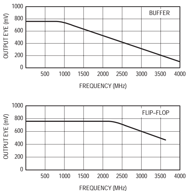
Figure 1. Eye Pattern versus Frequency
