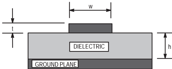
Figure 3.1. Microstrip Line
