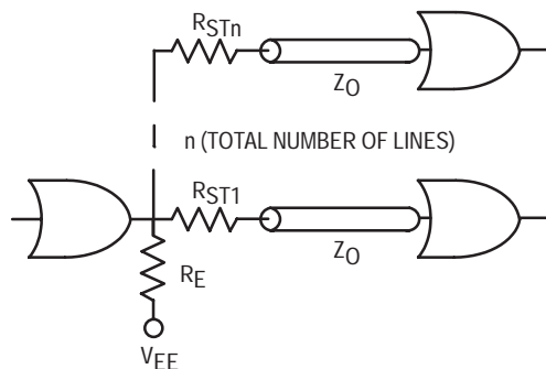
Figure 3.19. Parallel Fanout using Series Termination
