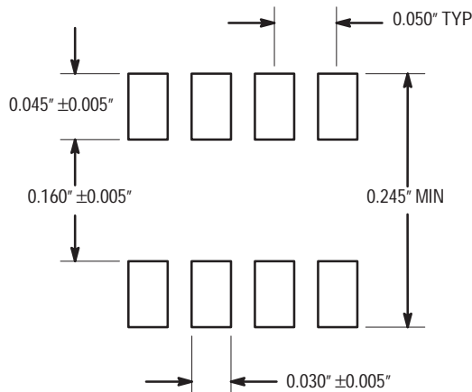
Figure 3. 8-, 16-Lead SOIC Solder Pad Dimensions
