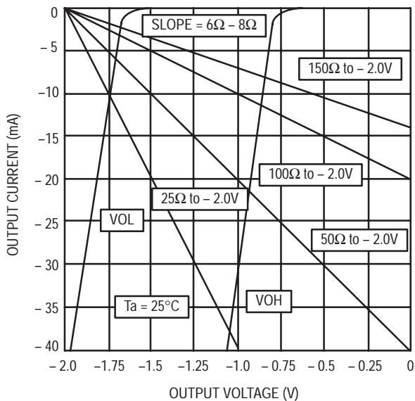
Figure 3.14. ECLINPS Output Characteristics
