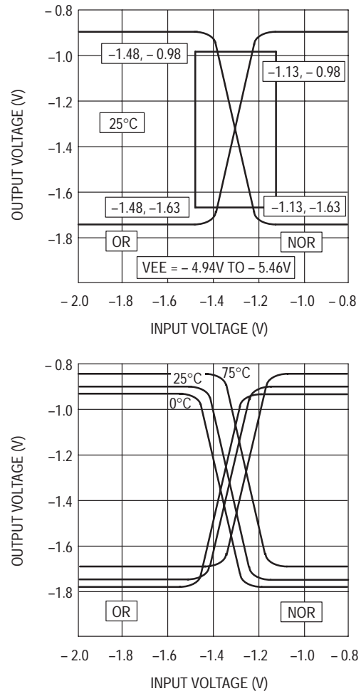
Figure 2.2. ECLinPS 10E Transfer Curves
