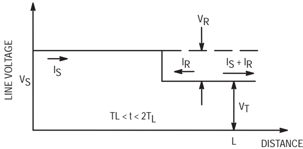
Figure 2.6. Reflected Voltage Wave for R_T < Z_0
