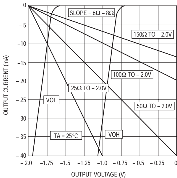
Figure 2.1. Output Characteristics vs Load
