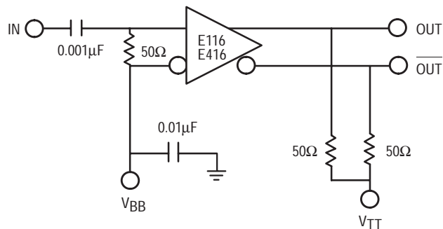
Figure 4.3. AC Couple Circuit
