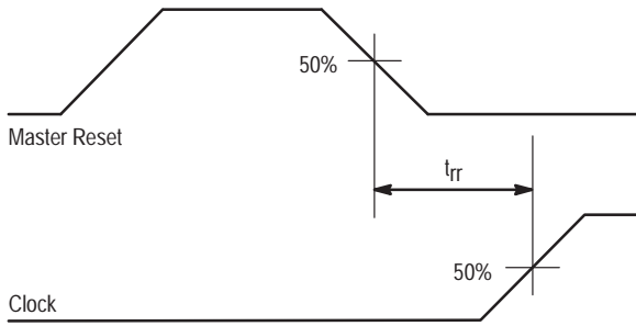
Figure 2.6. ECLinPS Release Time Waveforms
