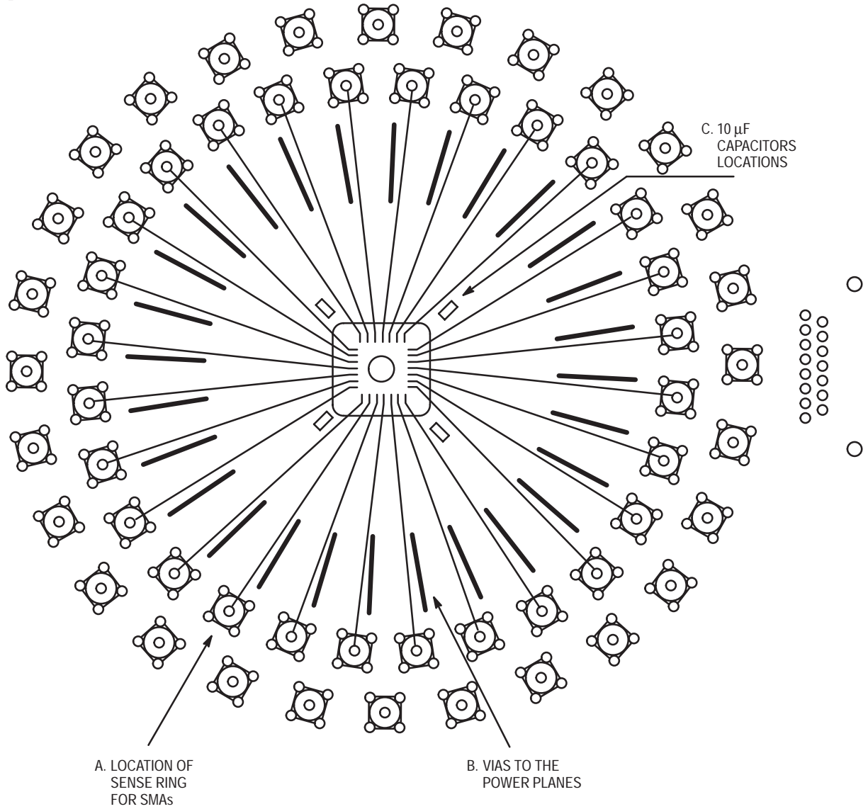
Figure 1. Front View of ECLinPS Evaluation Board
