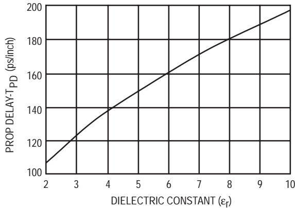
Figure 3.4. Propagation Delay vs Dielectric Constant
