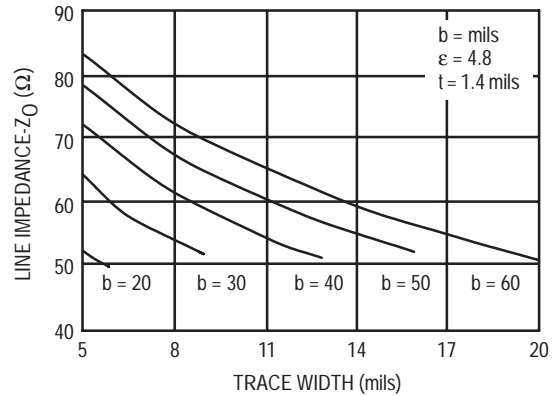
Figure 3.6. Stripline Impedance vs Trace Width
