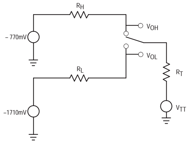
Figure 3.15. Equivalent Model for Calculating 10E Output Levels
