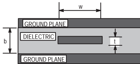
Figure 3.5. Stripline Structure
