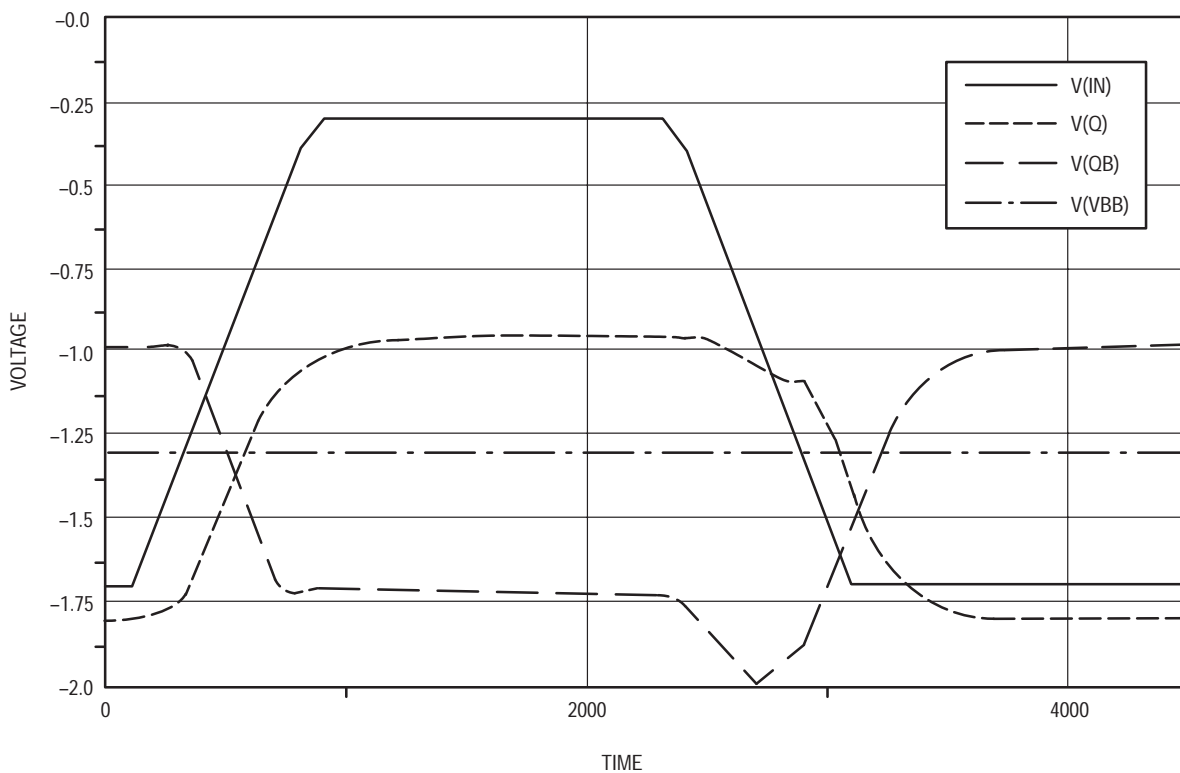
Figure 7. Input and Output Waveforms for V_{IH} = -0.3 ( V_{OL} = -1.8 ; T_{PD++} = 196\text{ps} ; T_{PD--} = 198\text{ps} ; I_{INH} = 114.8\mu\text{A} )
