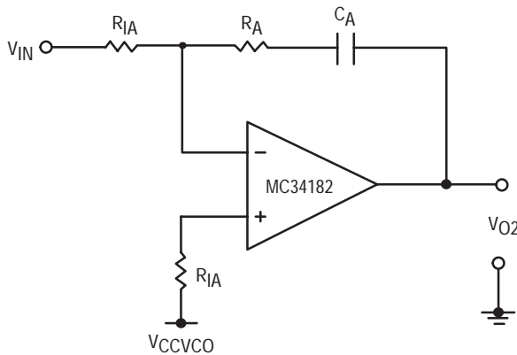
Figure 7. Integrator Subsection
