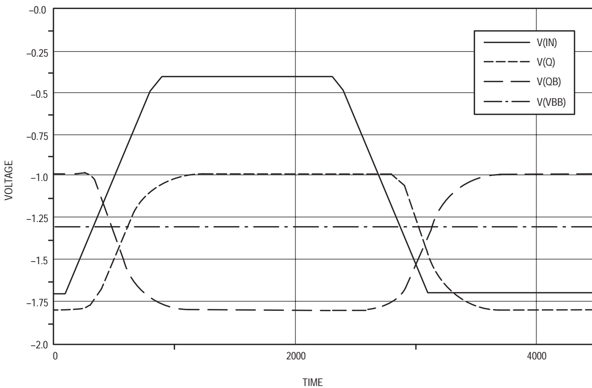
Figure 6. Input and Output Waveforms for V_{IH} = -0.4 ( V_{OL} = -1.8 ; T_{PD++} = 201\text{ps} ; T_{PD--} = 206\text{ps} ; I_{INH} = 46.7\mu\text{A} )
