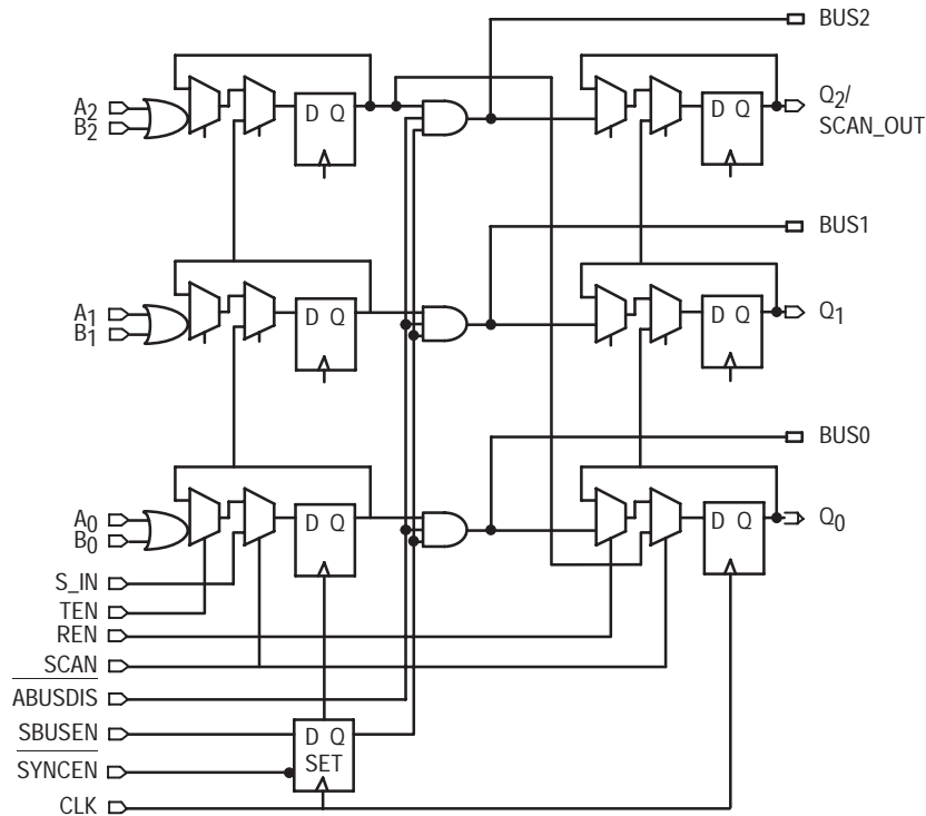
LOGIC DIAGRAM
