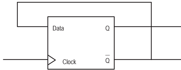
Figure 2.7. f MAX Measurement
