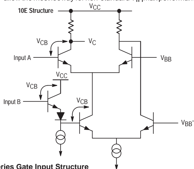
Figure 3. Emitter Follower Series Gate Input Structure
