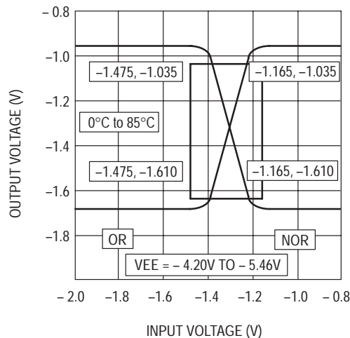
Figure 2.3. ECLinPS 100E Transfer Characteristics
