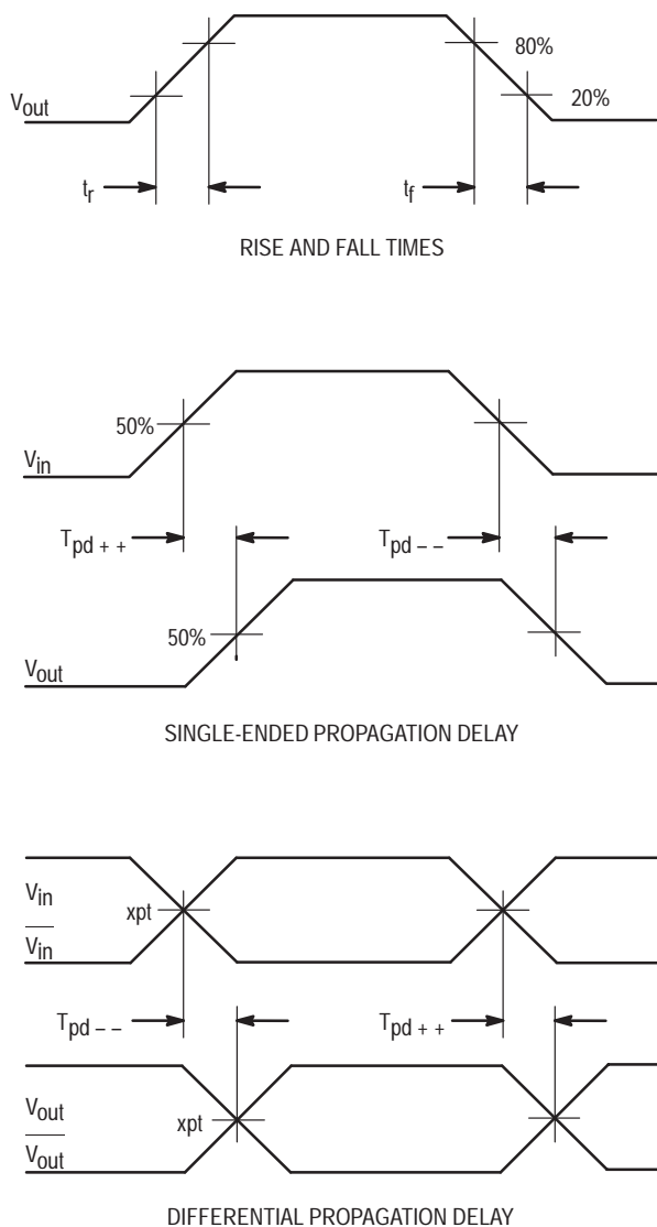
Figure 2.4. ECLinPS Tpd Measurement Waveforms
