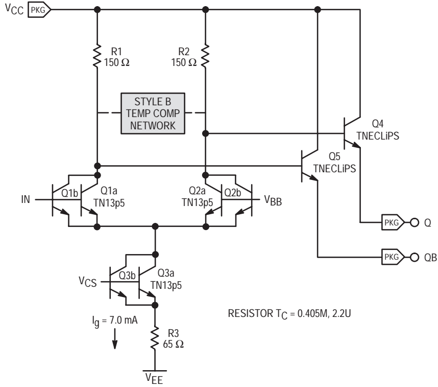
Figure 5. 2x Current Output Schematic
