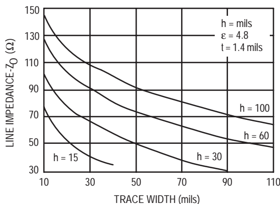
Figure 3.2. Microstrip Impedance vs Trace Width
