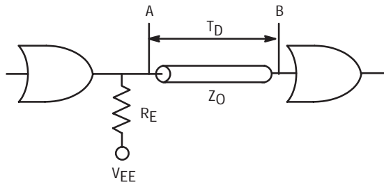
Figure 3.12. Unterminated Transmission Line
