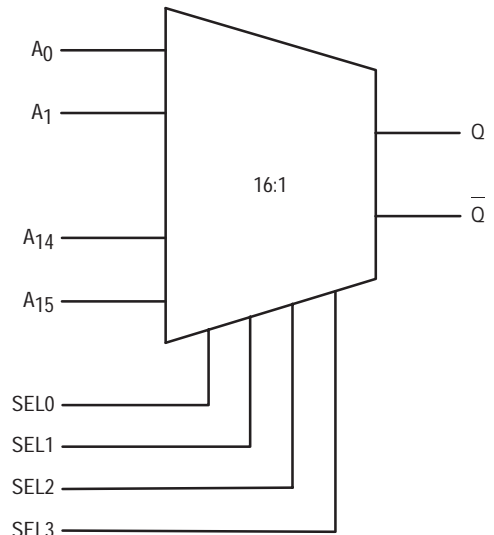
LOGIC DIAGRAM
