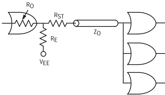
Figure 3.22. Noise Margin Loss Example
