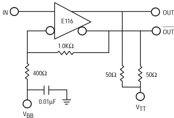
Figure 4.2. Schmitt Trigger w/100MV of Hysteresis
