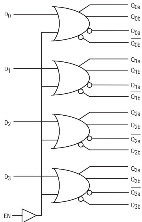
LOGIC DIAGRAM
