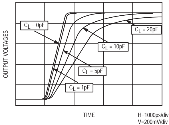
Figure 2.20. Line Delay vs Lumped Capacitive Load
