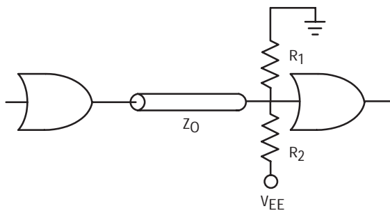
FIGURE 3.13B THEVENIN EQUIVALENT PARALLEL TERMINATION
