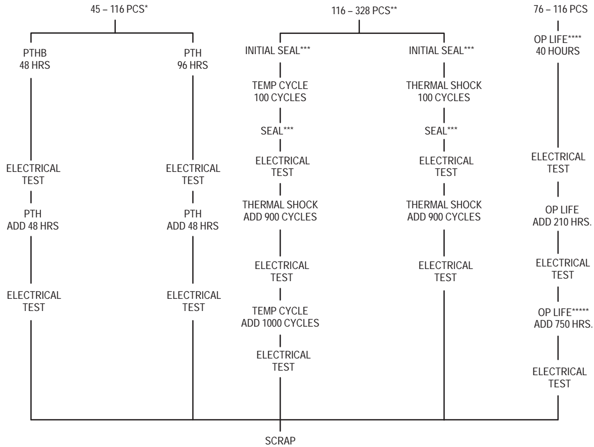
Figure 6.1. Reliability Audit Program Test Flow
