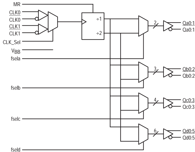
LOGIC SYMBOL
