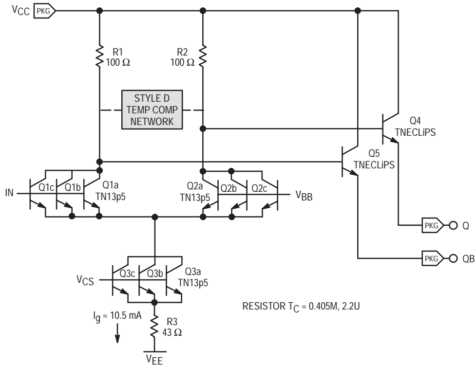
Figure 6. 3x Current Output Schematic
