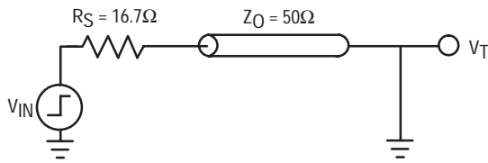
Figure 2.10. Transmission Line Model for Shorted Line
