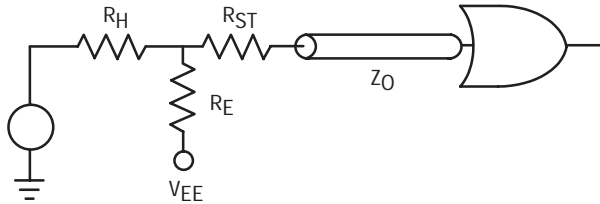
Figure 3.20. Equivalent Circuit for R_E Determination
