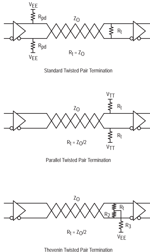
Figure 4. Twisted Pair Termination Techniques
