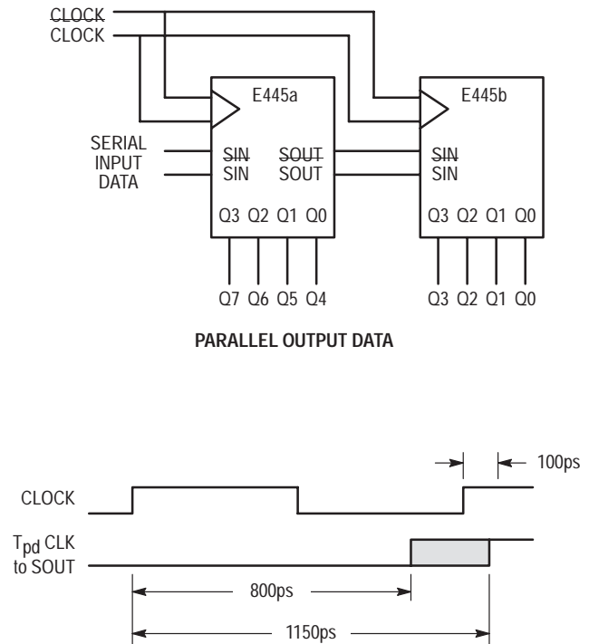
Figure 2. Cascaded 1:8 Converter Architecture
